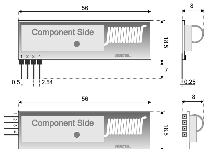
Mechanical Dimensions
