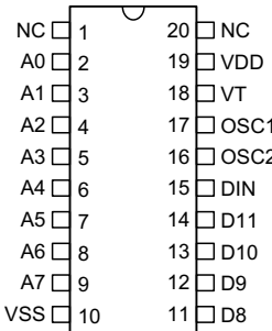
HT12D -20 SOP
