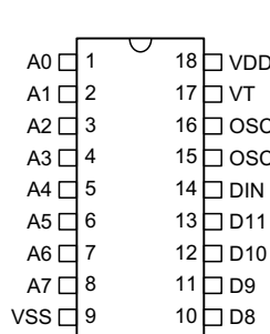
HT12D -18 DIP
