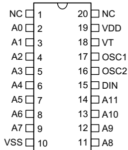
HT12F -20 SOP
