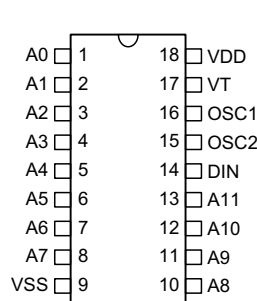
HT12F -18 DIP
