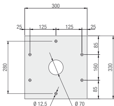
LOWER FASTENING BASE FOR: PSE3000 - PSU3000 - PSC3000
