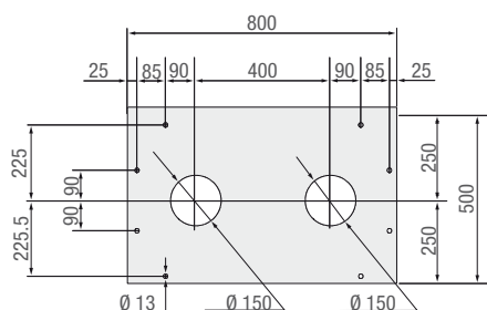
LOWER FASTENING BASE FOR: PSC7001
