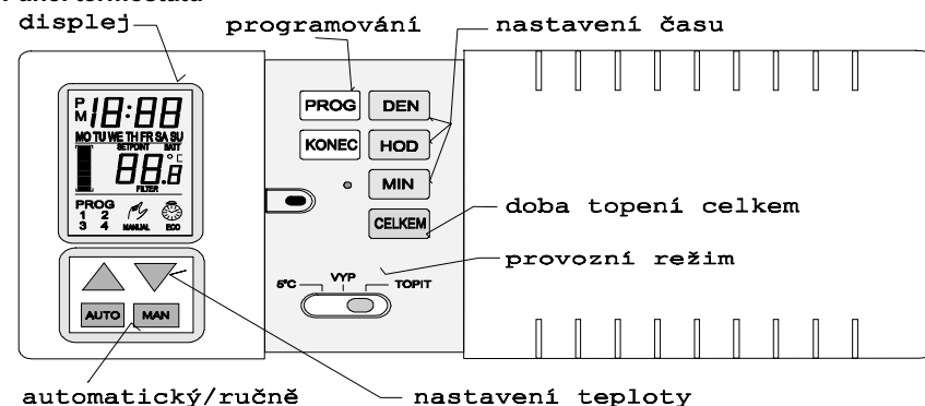
Obr. 1 Panel termostatu
